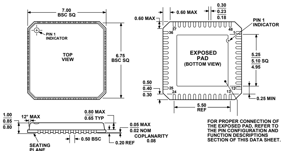
Figure 50. 48-Lead Lead Frame Chip Scale Package [LFCSP_VQ] 7 mm × 7 mm Body, Very Thin Quad (CP-48-1)
