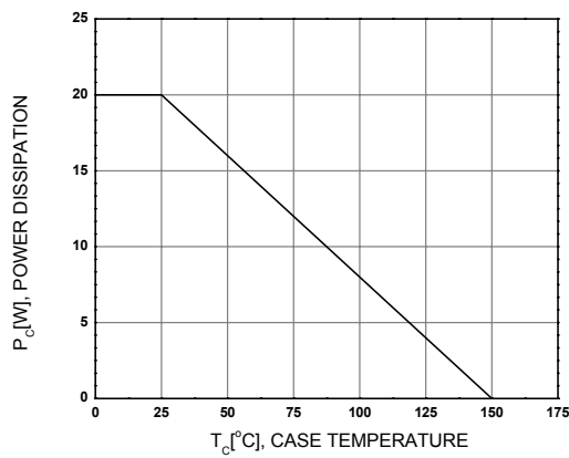
Figure 3. Power Derating vs T_C
