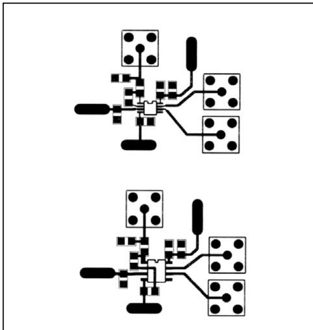
Figure 5. MAX961 PCB Layout
