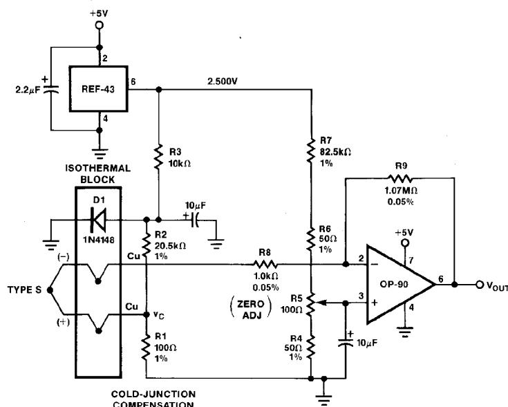
FIGURE 9: Thermocouple Amplifier with Cold-Junction Compensation
