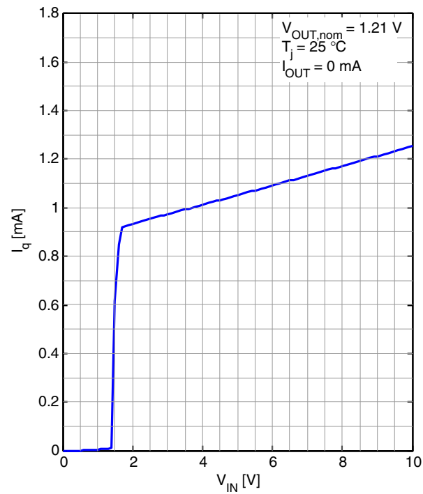
Quiescent Current I_q versus Input Voltage V_{IN} ( V_{OUT,nom} = 1.21 \text{ V} )
