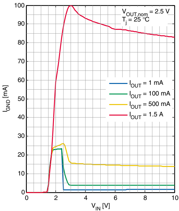
GND Pin Current I_{\text{GND}} versus Input Voltage V_{\text{IN}} ( V_{\text{OUT,nom}} = 2.5 \text{ V} )
