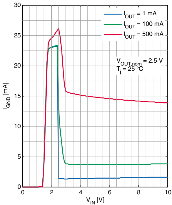
GND Pin Current I_{\text{GND}} versus Input Voltage V_{\text{IN}} ( V_{\text{OUT,nom}} = 2.5 \text{ V} )
