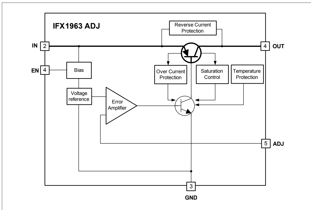
Figure 1 Block Diagram
