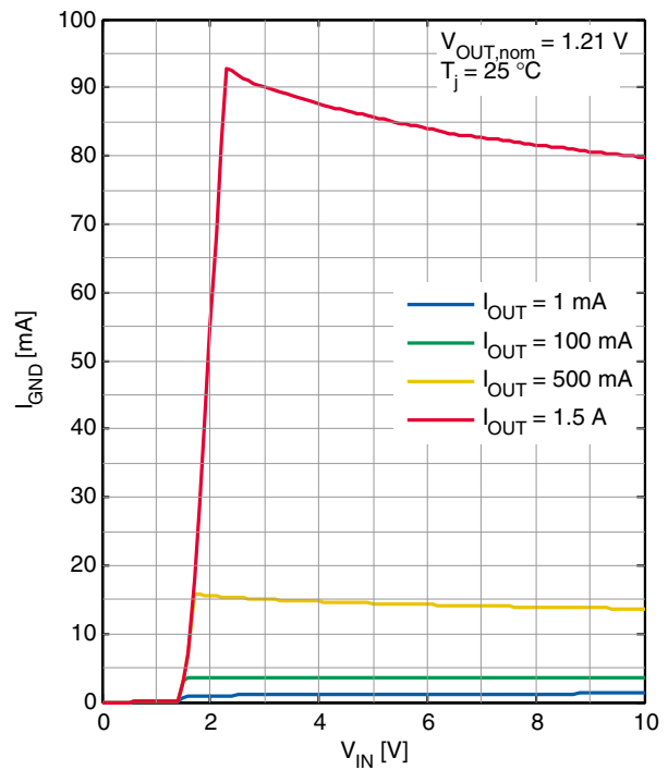
GND Pin Current I_{\text{GND}} versus Input Voltage V_{\text{IN}} ( V_{\text{OUT,nom}} = 1.21 \text{ V} )
