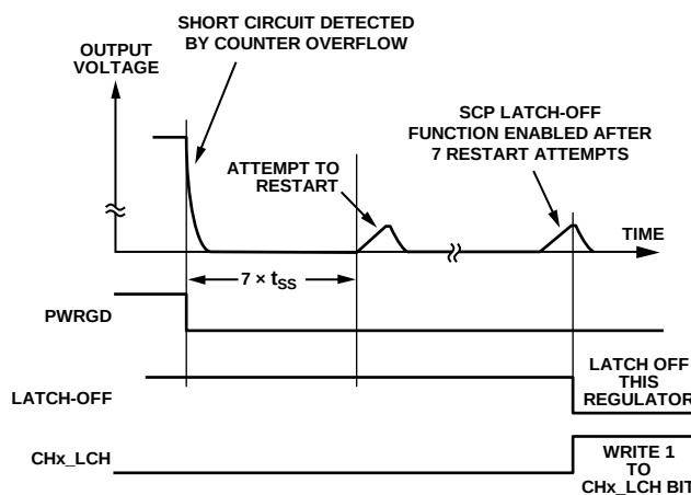
Figure 52. Short-Circuit Latch-Off Detection
