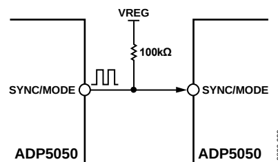
Figure 47. Two ADP5050 Devices Configured for Synchronization Mode
