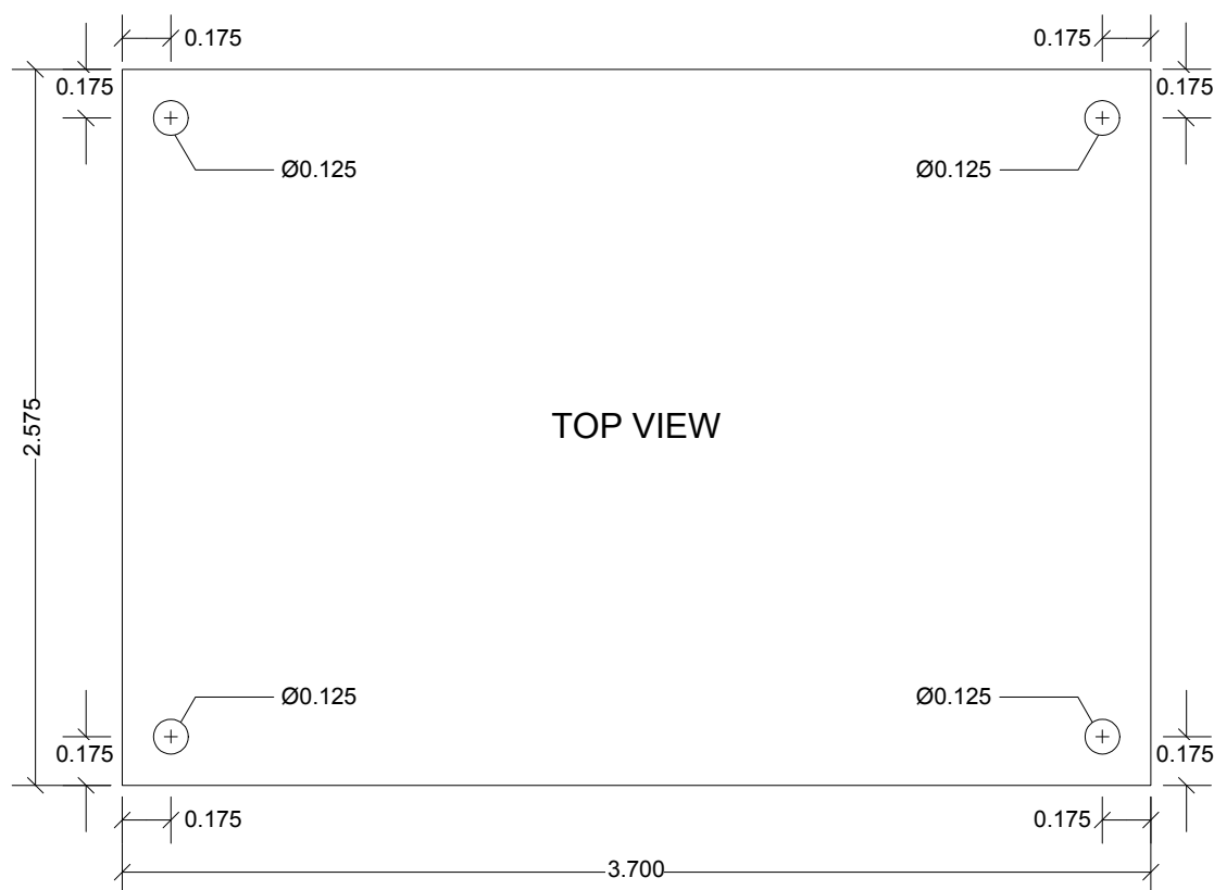
Figure 2.2 EVB-LAN9730-MII Mechanicals
