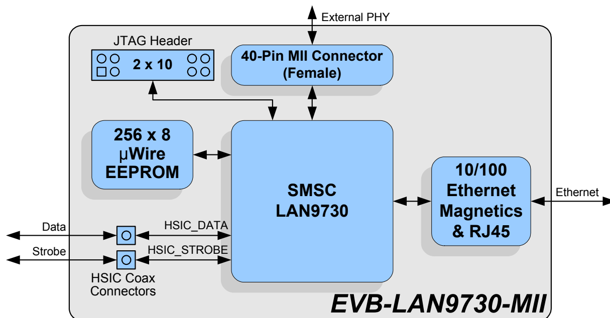
Figure 1.1 EVB-LAN9730-MII Block Diagram
