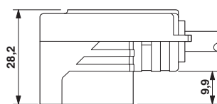
Valve connector, type BI, side view
