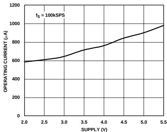
Figure 16. Operating Current vs. Supply
