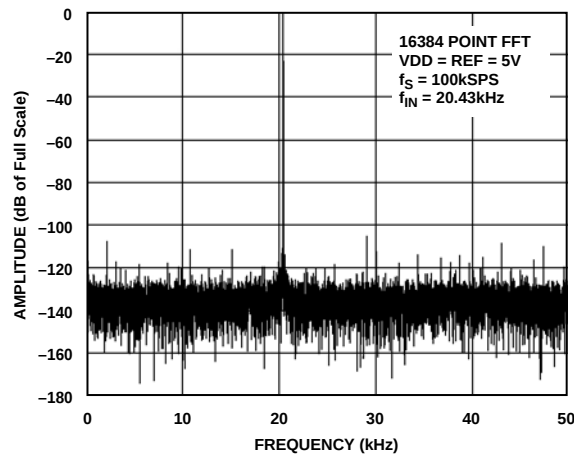
Figure 9. FFT Plot
