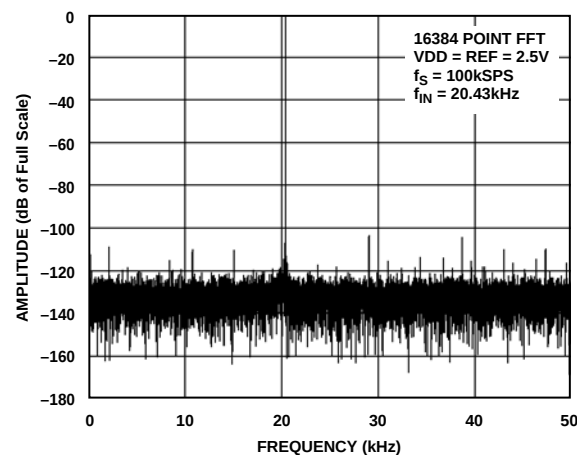
Figure 12. FFT Plot
