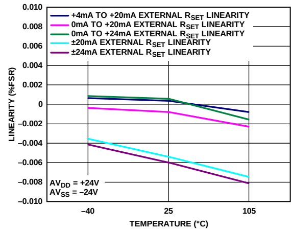
Figure 33. INL vs. Temperature, External R_{SET} Sense Resistor
