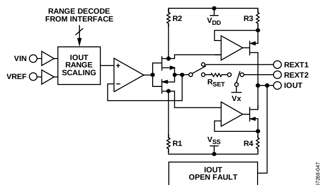
Figure 53. Current Output Configuration
