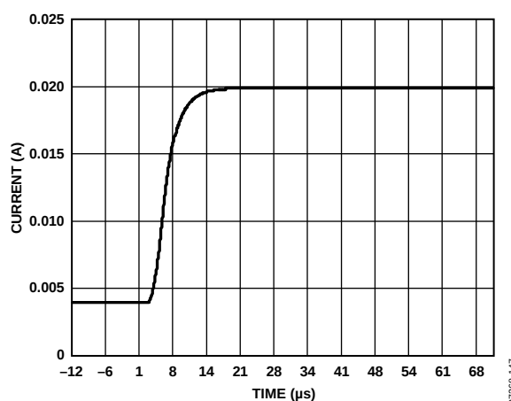
Figure 47. 4 mA to 20 mA Output Current Step
