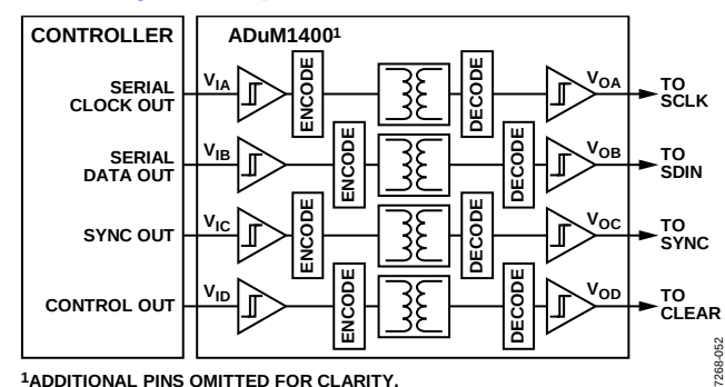
Figure 58. Isolated Interface
