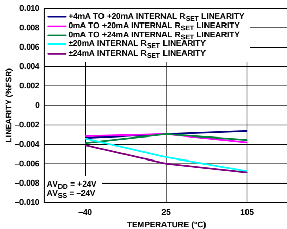
Figure 32. INL vs. Temperature, Internal R_{SET} Sense Resistor
