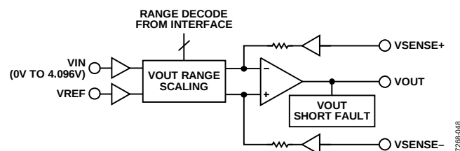
Figure 54. Voltage Output
