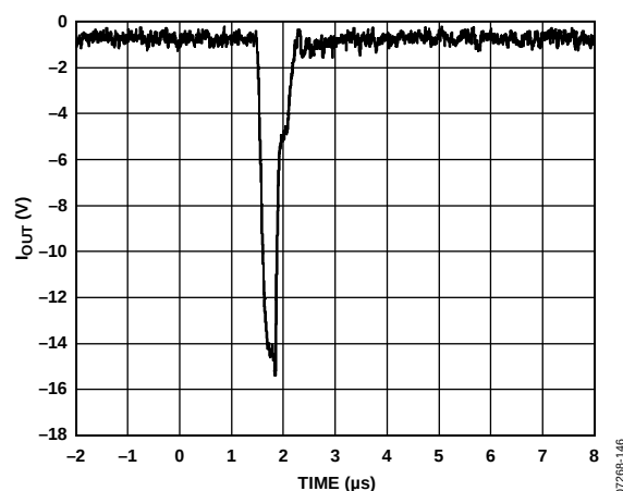
Figure 46. Output Current ( I_{OUT} ) vs. Time-On Output Enable
