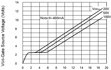
Gate charge v gate-source voltage
