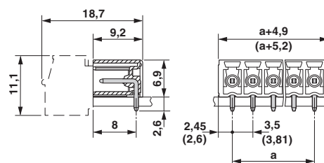
Dimensioned drawing
