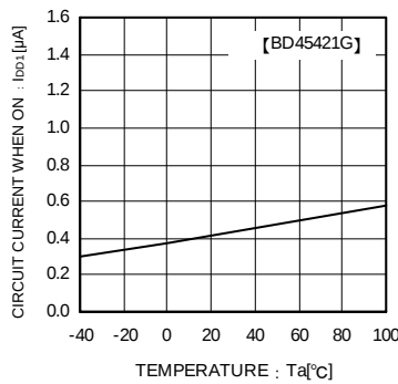
Fig.10 Circuit Current when ON ( V_{DET}=0.2\text{V} )
