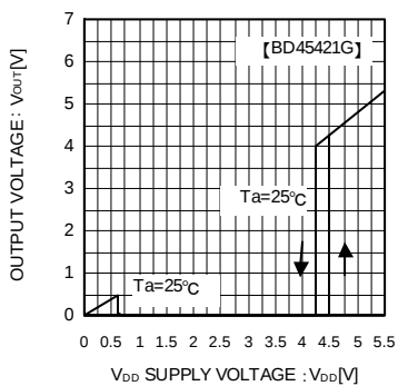
Fig.6 I/O Characteristics
