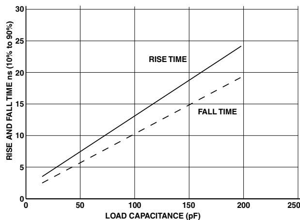
Figure 46. Typical Output Rise and Fall Times (10% to 90%) vs. Load Capacitance for Driver C at V_{DDEXT} = 2.7 V (Min)
