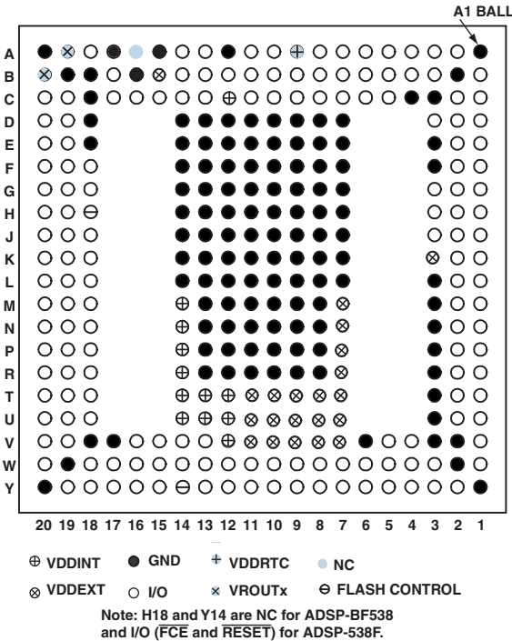
Figure 53. 316-Ball CSP_BGA Ball Configuration (Bottom View)
