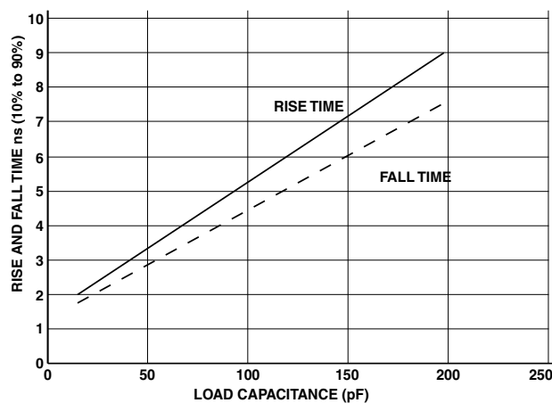
Figure 45. Typical Output Rise and Fall Times (10% to 90%) vs. Load Capacitance for Driver B at V_{DDEXT} = 3.6 V (Max)
