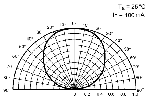
Fig. 8.7 Radiation Pattern
