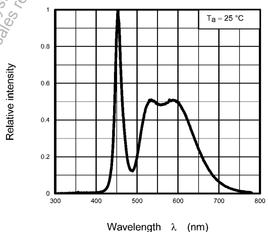
Fig. 8.6 Wavelength Characteristic
