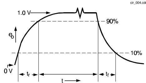
SWITCHING WAVEFORM
