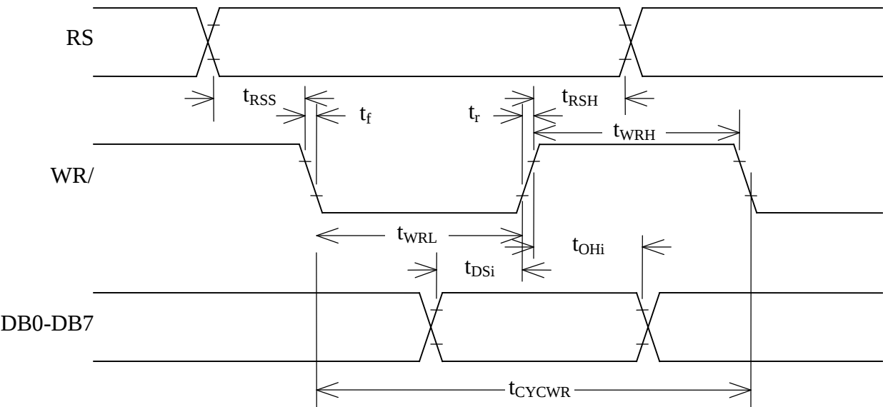
Figure 3. Intel I80-Typte Parallel Interface Write Cycle Timing
