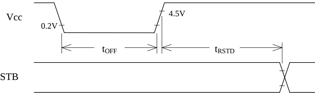
Figure 7. Power-Up Internal Reset Timing
