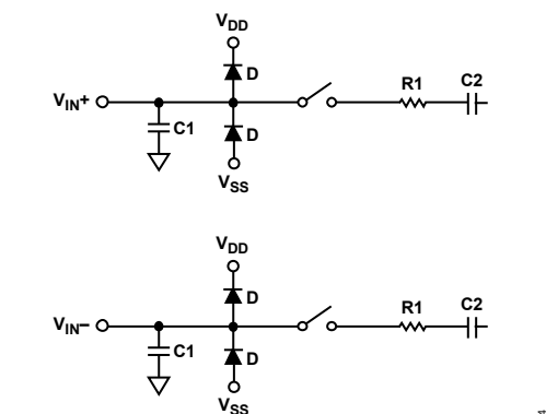
NOTES 1. V_{IN+} CAN BE V_{IN0} OR V_{IN2} , AND V_{IN-} CAN BE V_{IN1} OR V_{IN3} . Figure 30. Equivalent Analog Input Circuit (Differential)
