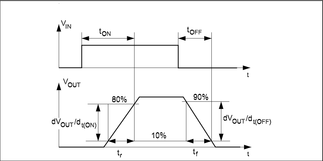
Figure 4. Switching characteristics
