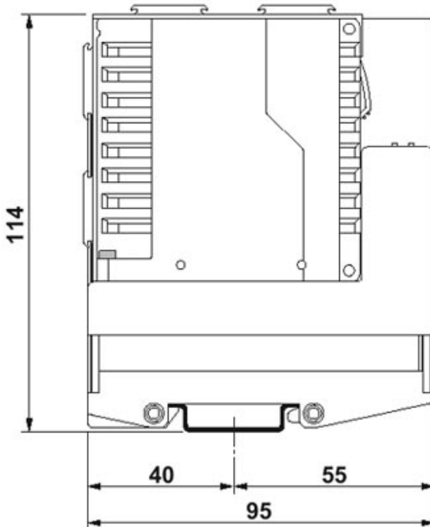
Dimensioned drawing
