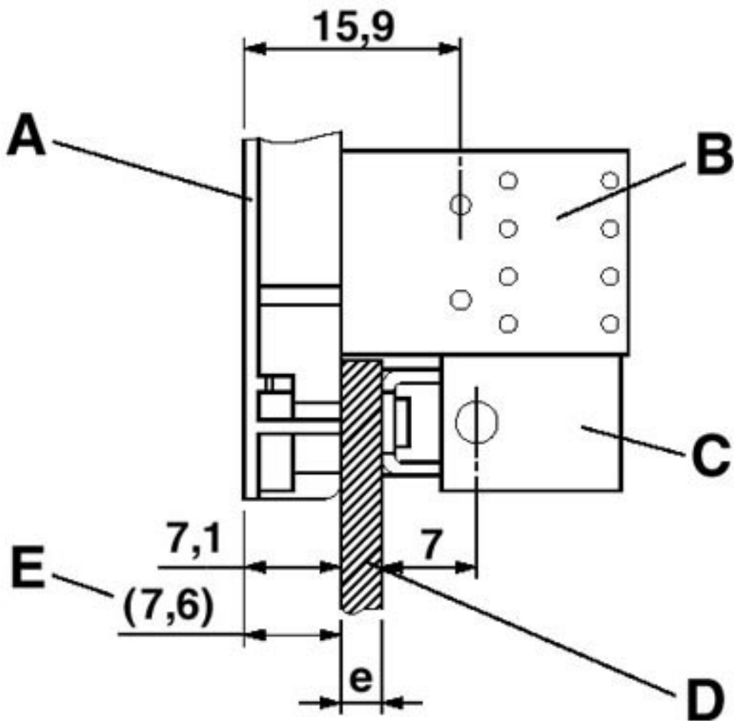
Dimensioned drawing
