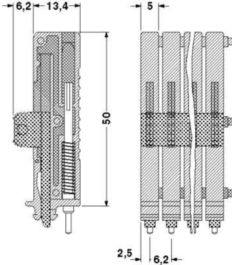
Dimensioned drawing
