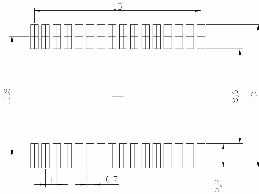
Figure 14. SCR1100 footprint.
