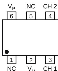
Pin Configuration
