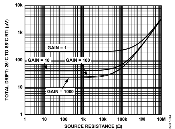
Figure 14. Total Drift vs. Source Resistance
