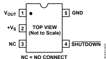
Figure 2. R-5 (SOT-23)
