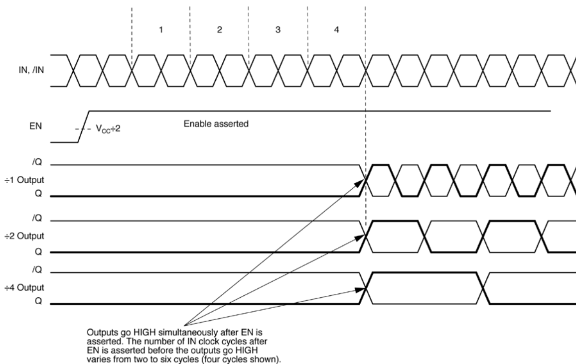
Timing Diagram Showing Enable Timing
