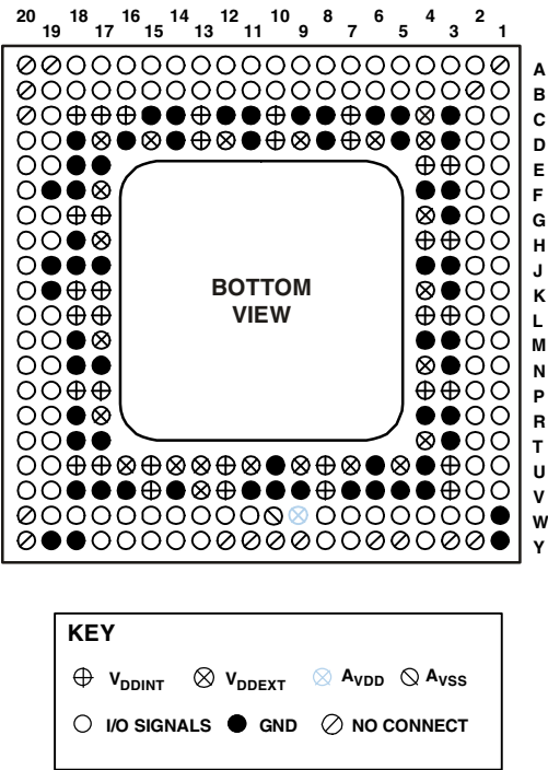
Figure 48. 256-Ball BGA_ED Ball Configuration (Bottom View)
