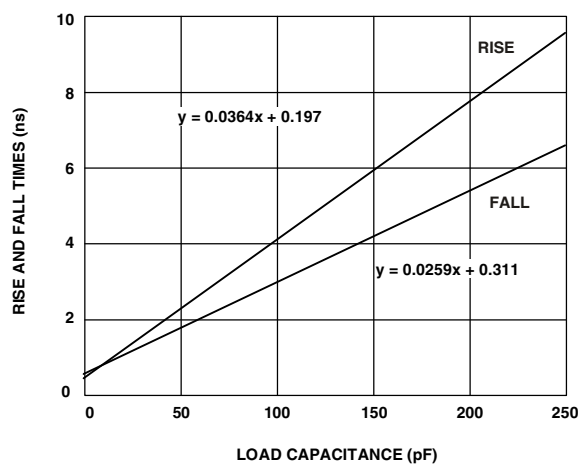
Figure 45. SDCLK Typical Output Rise/Fall Time (20% to 80%, V_{DDEXT} = \text{Max} )
