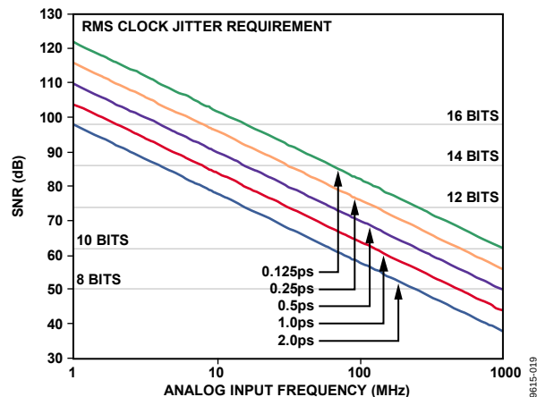
Figure 35. Ideal SNR vs. Input Frequency and Jitter
