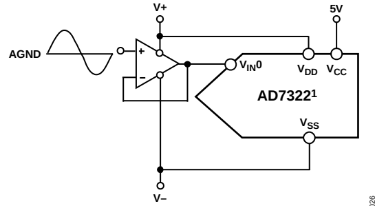
Figure 33. Single-Ended Mode Typical Connection Diagram
