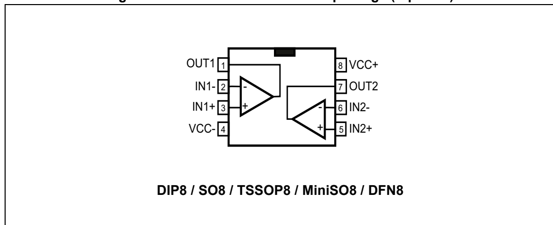
Figure 2. Pin connections for each package (top view)
