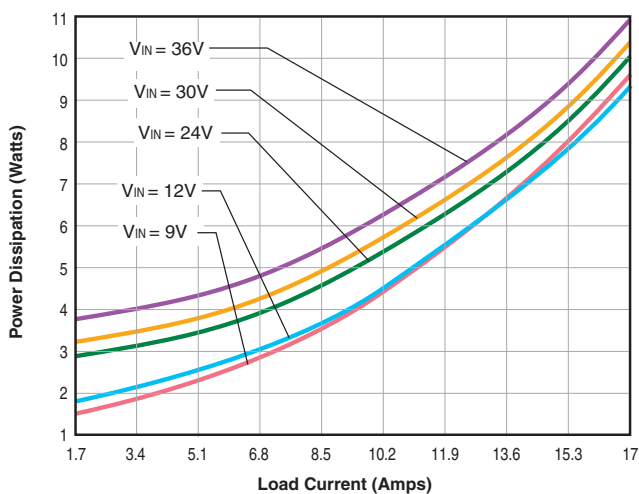
UQQ-5/17-Q12P Power Dissipation vs. Load Current @ 25°C
