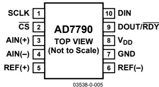
Figure 5. Pin Configuration
