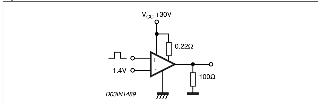
Figure 14. Test circuit
