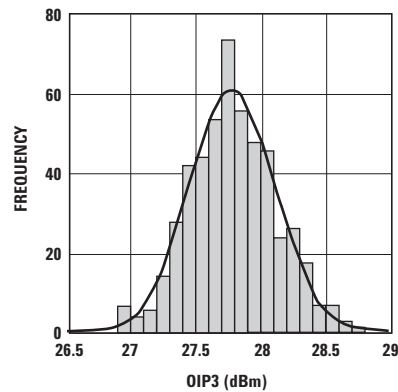
Figure 4. OIP3 Distribution.
