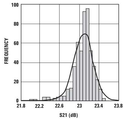
Figure 1. S21 Distribution.
