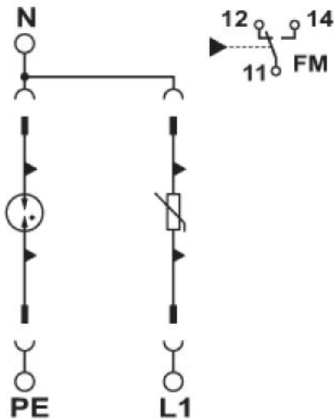
Circuit diagram
