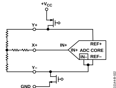
Figure 22. Differential Reference Mode ( SER/DFR = 0 )
