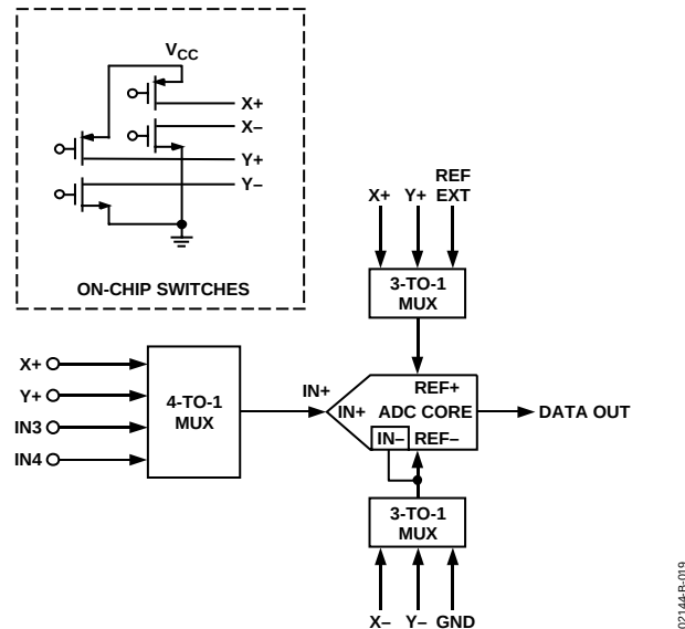
Figure 19. Equivalent Analog Input Circuit
