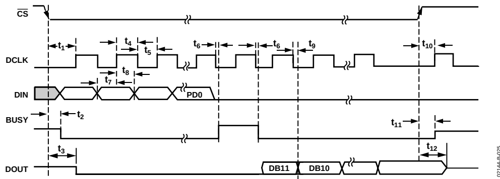
Figure 25. Detailed Timing Diagram
