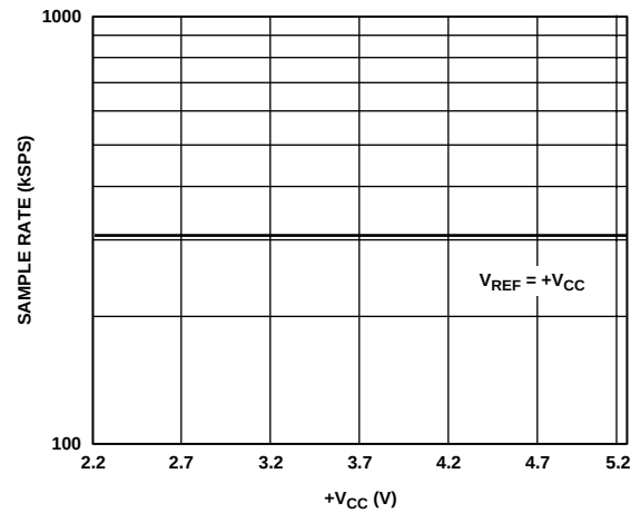
Figure 8. Maximum Sample Rate vs. +V_{\text{CC}}
