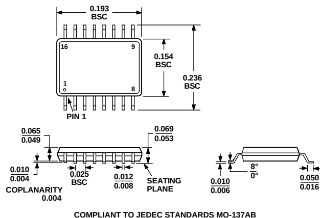
Figure 30. 16-Lead Shrink Small Outline Package [QSOP] (RQ-16) Dimensions shown in inches
