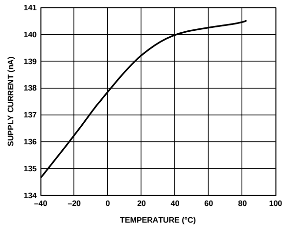
Figure 7. Power-Down Supply Current vs. Temperature
