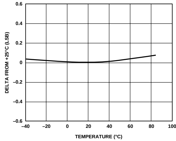
Figure 9. Change in Offset vs. Temperature
