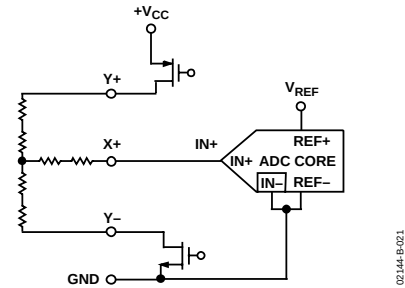
Figure 21. Single-Ended Reference Mode ( SER/DFR = 1 )
