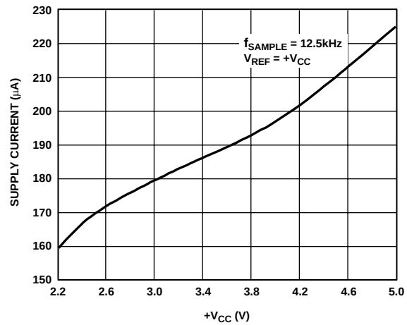
Figure 5. Supply Current vs. +V_{\text{CC}}
