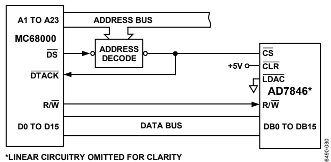
Figure 28. AD7846-to-MC68000 Interface
