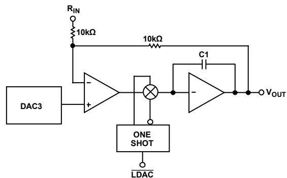
Figure 22. Output Stage
