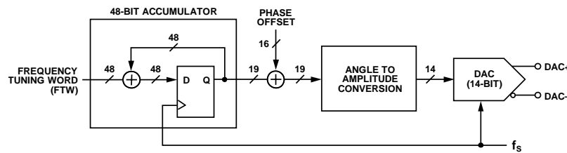
Figure 41. DDS Block Diagram
