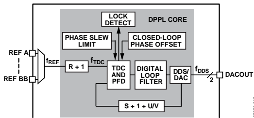
Figure 36. Digital PLL Core
