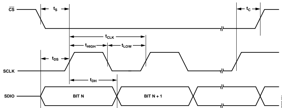
Figure 58. Serial Control Port Timing—Write
