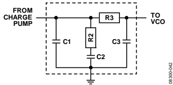
Figure 66. Third-Order Analog Loop Filter
