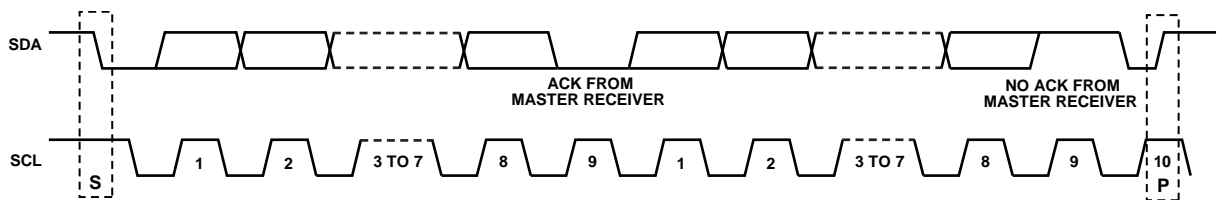
Figure 63. Data Transfer Process (Master Read Mode, 2-Byte Transfer Used for Illustration)
