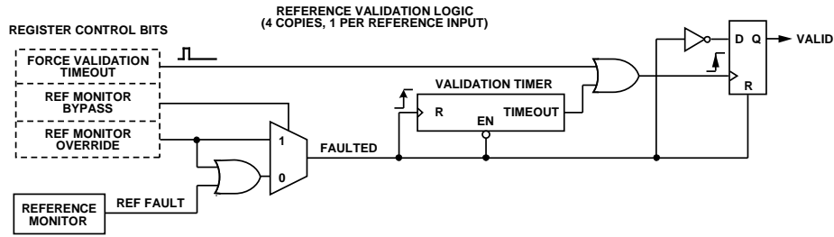
Figure 33. Reference Validation Override
