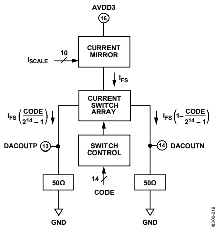
Figure 42. DAC Output Pins
