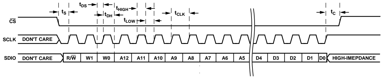
Figure 54. Serial Control Port Read—MSB First, 16-Bit Instruction, One Byte of Data
