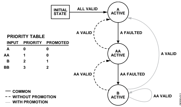
Figure 34. Example of Priority Promotion
