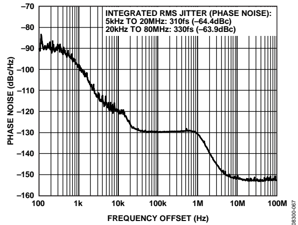
Figure 6. Additive Phase Noise (Output Driver = LVPECL), f_{REF} = 19.44 MHz, f_o = 311.04 MHz, LBW = 1 kHz, f_{SYSCLK} = 50 MHz (Crystal), PLL On
