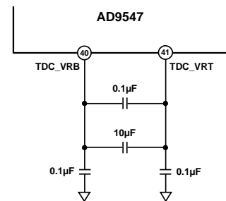
Figure 37. TDC Pin Connections
