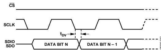
Figure 56. Serial Control Port Timing—Read
