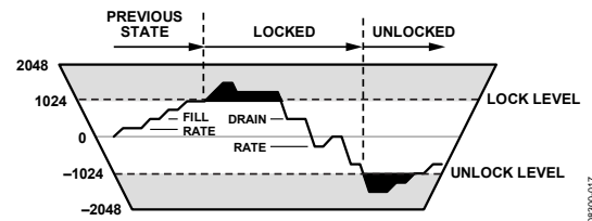
Figure 40. Phase Lock Detector Diagram
