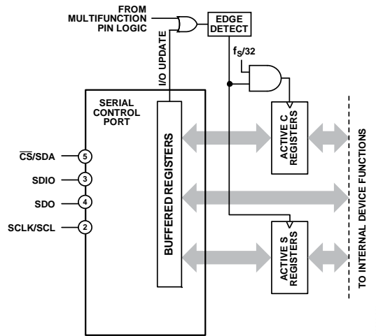
Figure 65. Buffered and Active Registers
