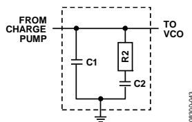
Figure 67. Second-Order Analog Loop Filter
