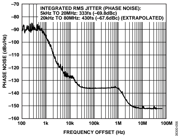
Figure 4. Additive Phase Noise (Output Driver = LVPECL), f_{REF} = 19.44 MHz, f_o = 155.52 MHz, LBW = 1 kHz, f_{SYSCLK} = 50 MHz (Crystal), PLL On
