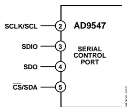
Figure 51. Serial Control Port
