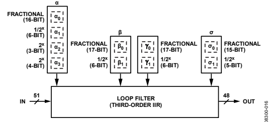
Figure 39. Third-Order Digital IIR Loop Filter
