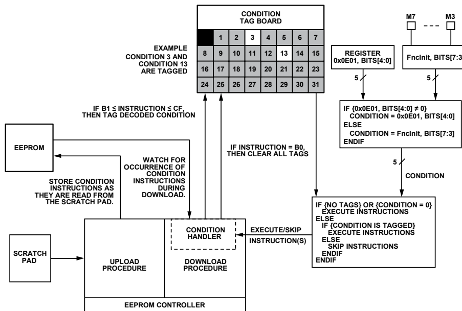
Figure 49. EEPROM Conditional Processing
