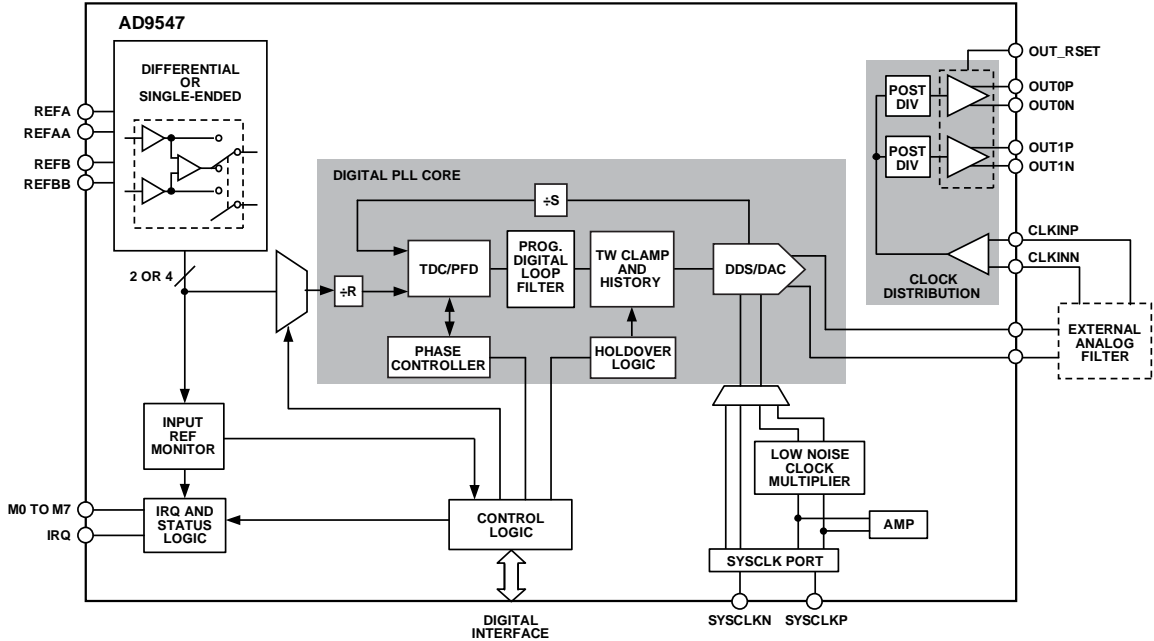
Figure 32. Detailed Block Diagram
