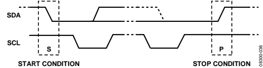
Figure 60. Start and Stop Condition
