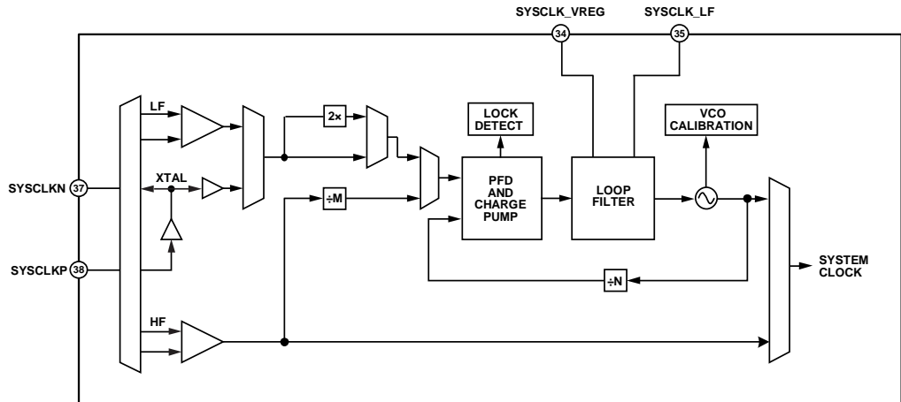
Figure 44. System Clock Block Diagram
