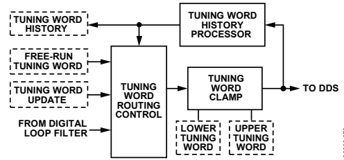
Figure 43. Tuning Word Processing
