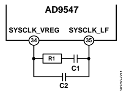
Figure 45. External Loop Filter Schematic
