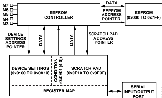
Figure 48. EEPROM Functional Diagram
