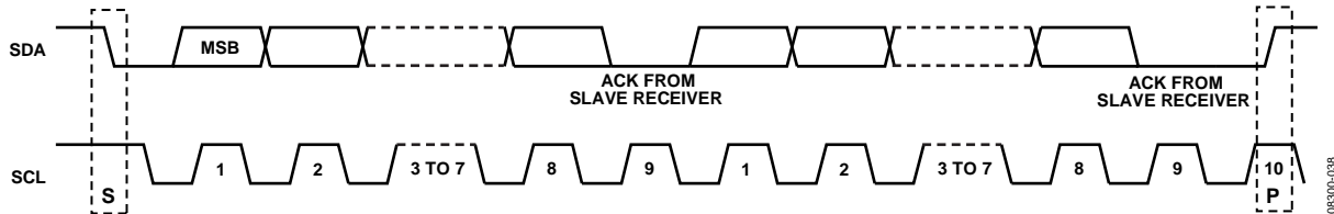
Figure 62. Data Transfer Process (Master Write Mode, 2-Byte Transfer Used for Illustration)
