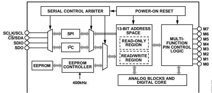
Figure 50. Serial Port Functional Diagram
