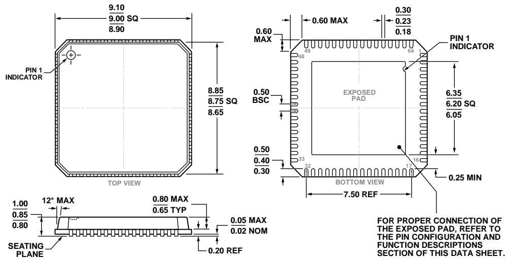
Figure 68. 64-Lead Lead Frame Chip Scale Package [LFCSP_VQ] 9 mm × 9 mm Body, Very Thin Quad (CP-64-4) Dimensions shown in millimeters
