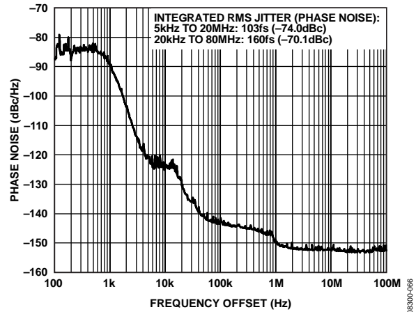
Figure 5. Additive Phase Noise (Output Driver = LVPECL), f_{REF} = 19.44 MHz, f_o = 311.04 MHz, LBW = 1 kHz, f_{SYSCLK} = 1 GHz, PLL Off
