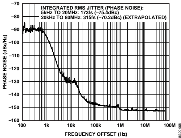
Figure 3. Additive Phase Noise (Output Driver = LVPECL), f_{REF} = 19.44 MHz, f_o = 155.52 MHz, LBW = 1 kHz, f_{SYSCLK} = 1 GHz, PLL Off
