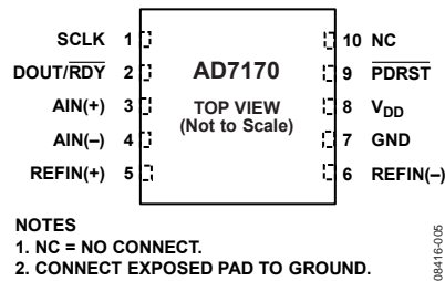
Figure 5. Pin Configuration
