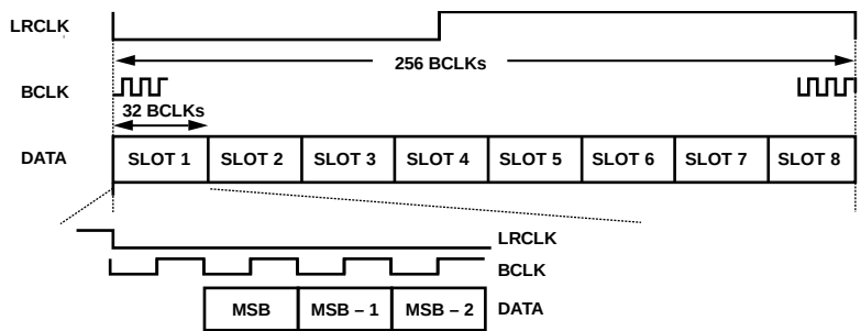
Figure 49. TDM Mode
