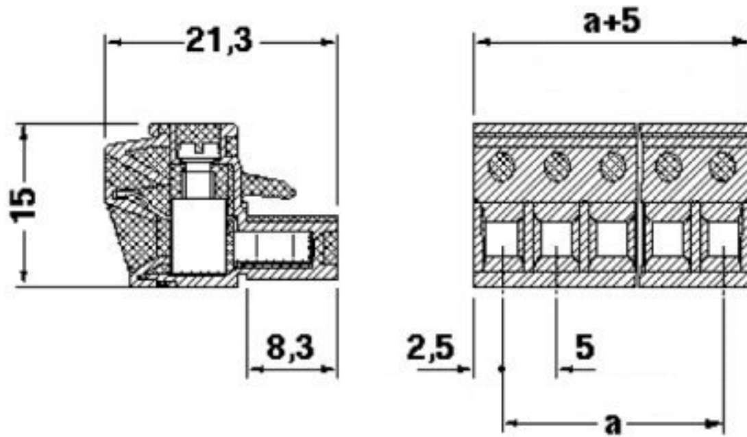
Dimensioned drawing
