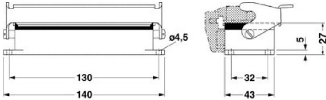
Dimensioned drawing
