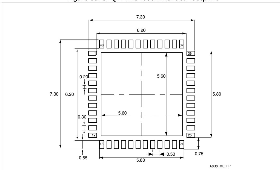
Figure 33. UFQFPN48 recommended footprint
