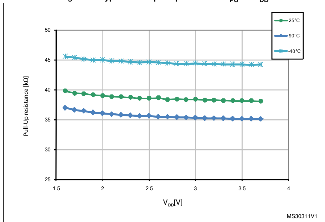
Figure 26. Typical NRST pull-up resistance R_{PU} vs. V_{DD}
