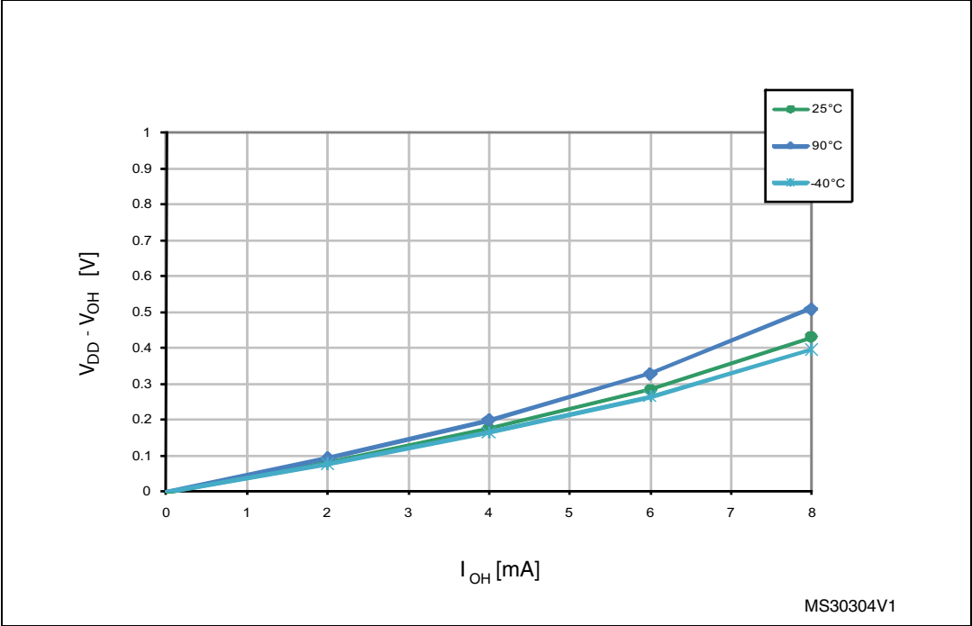
Figure 22. Typ. V_{DD} - V_{OH} at V_{DD} = 1.8\text{ V} (standard ports)
