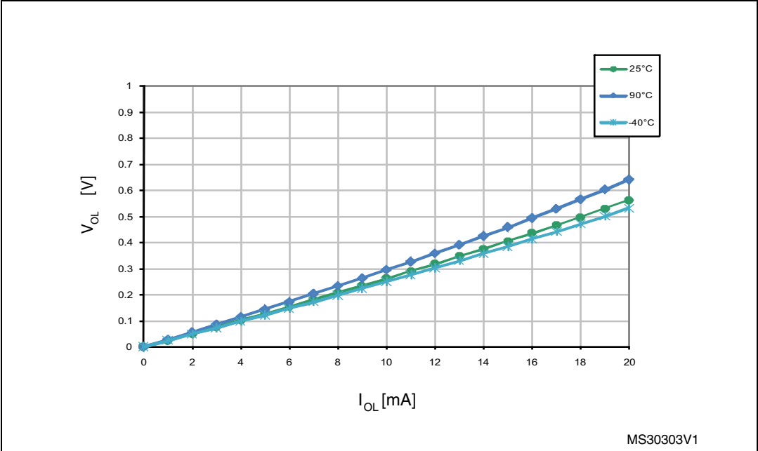
Figure 21. Typ. V_{OL} at V_{DD} = 3.0\text{ V} (standard ports)
