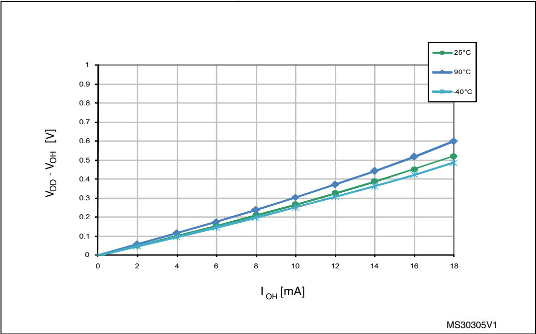
Figure 23. Typ. V_{DD} - V_{OH} at V_{DD} = 3.0\text{ V} (standard ports)
