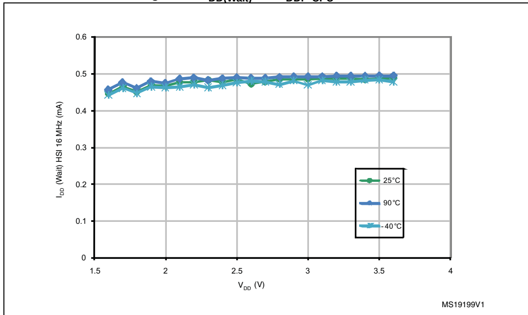
Figure 13. I_{DD}(\text{Wait}) vs. V_{DD} . f_{CPU} = 16 \text{ MHz}
