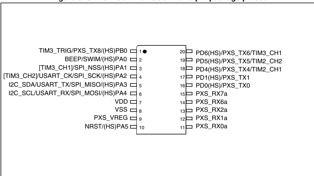
Figure 5. STM8TL53F4P6 TSSOP20 20-pin package pinout
