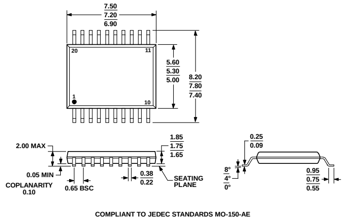
Figure 20. 20-Lead Shrink Small Outline Package [SSOP] (RS-20) Dimensions shown in millimeters
