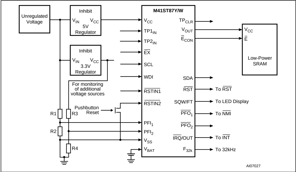
Figure 5. Hardware Hookup
