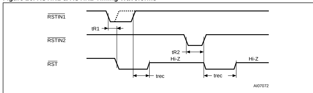
Figure 26. \overline{RSTIN1} & \overline{RSTIN2} Timing Waveforms
