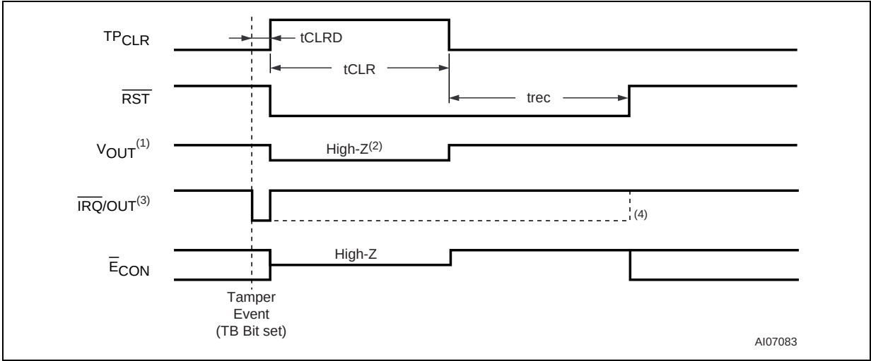
Figure 19. Tamper Output Timing (with CLR1EXT or CLR2EXT = '1')
