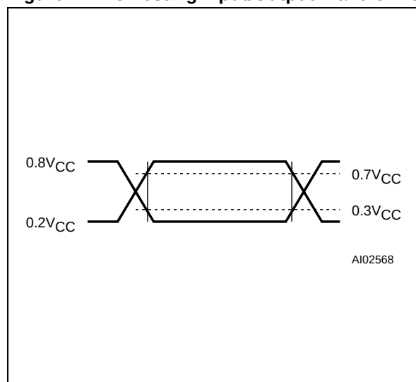
Figure 27. AC Testing Input/Output Waveforms
