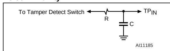
Figure 21. Low Pass Filter Implementation for Noise Immunity
