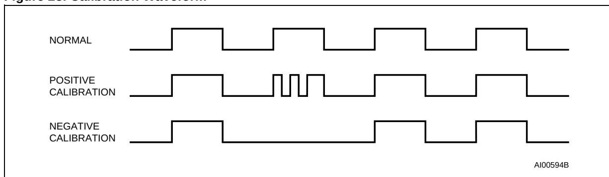
Figure 23. Calibration Waveform
