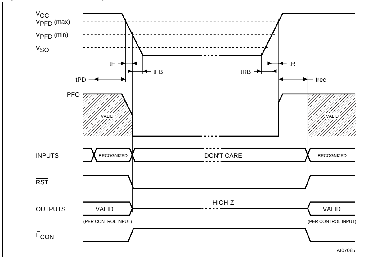
Figure 28. Power Down/Up Mode AC Waveforms
