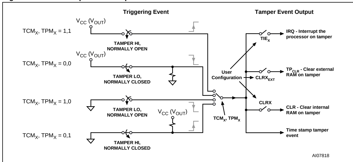
Figure 16. Basic Tamper Detect Options
