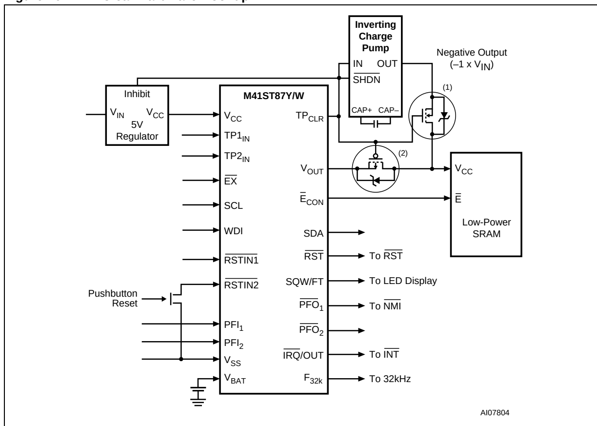
Figure 20. RAM Clear Hardware Hookup
