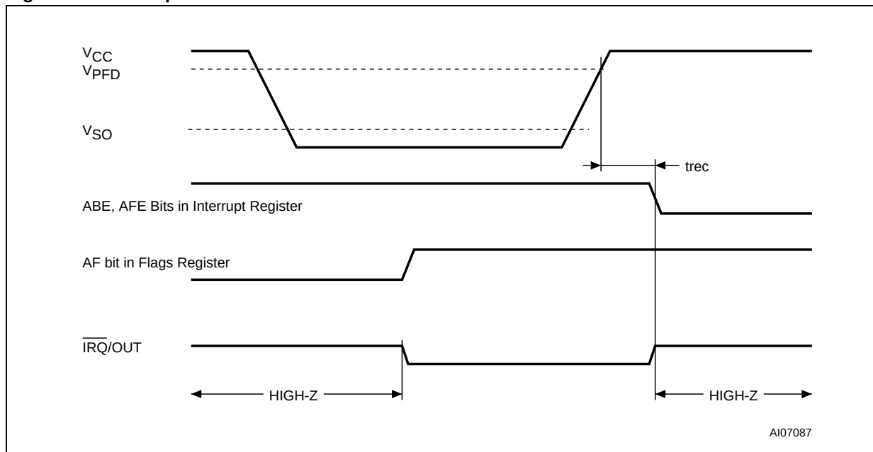
Figure 25. Back-Up Mode Alarm Waveform
