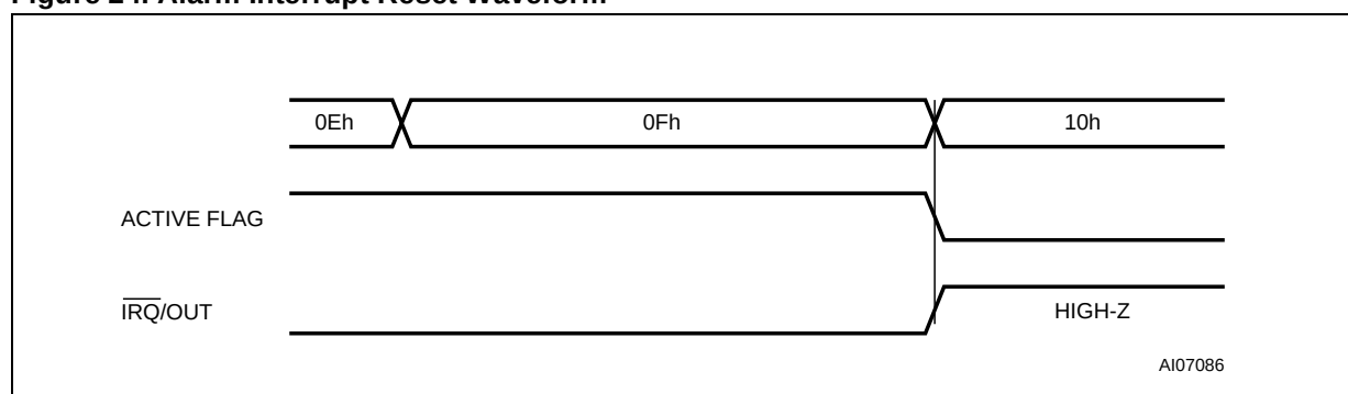
Figure 24. Alarm Interrupt Reset Waveform
