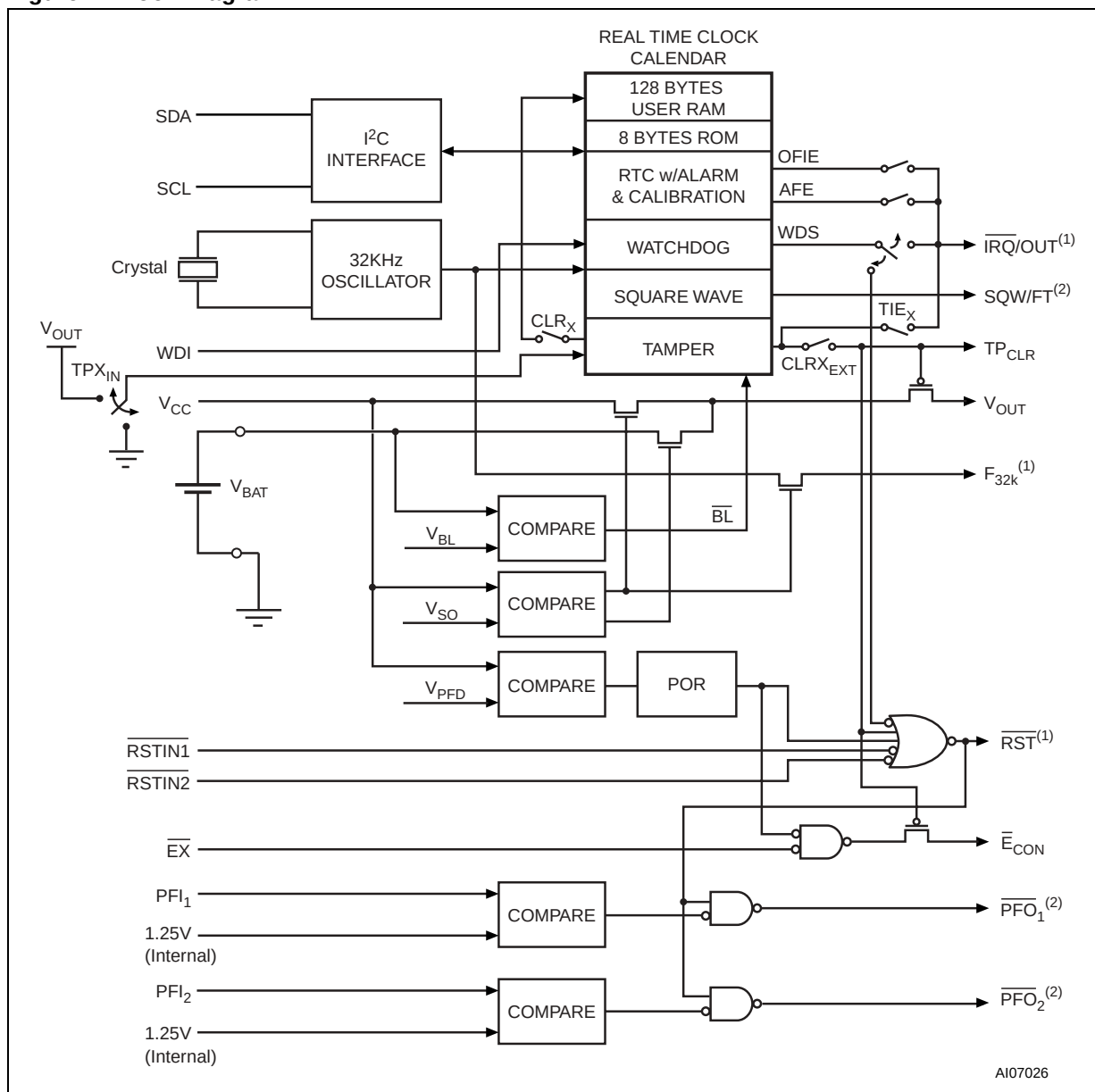
Figure 4. Block Diagram
