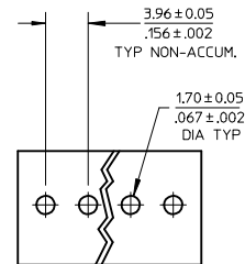
PCB LAYOUT: COMPONENT SIDE
