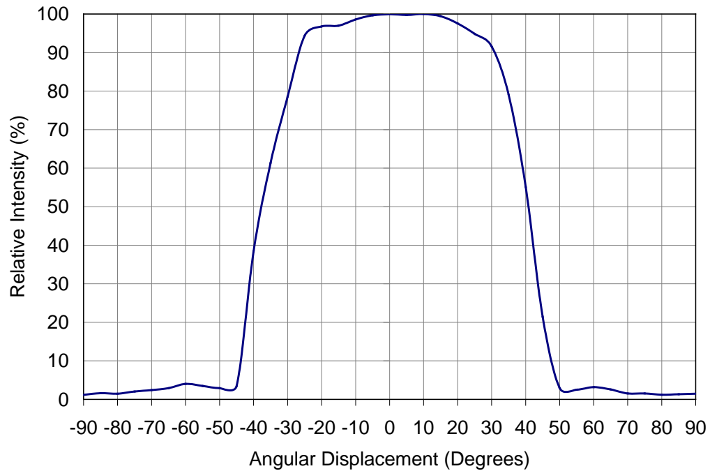
Figure 4: Typical representative spatial radiation pattern @ T c = 25°C.
