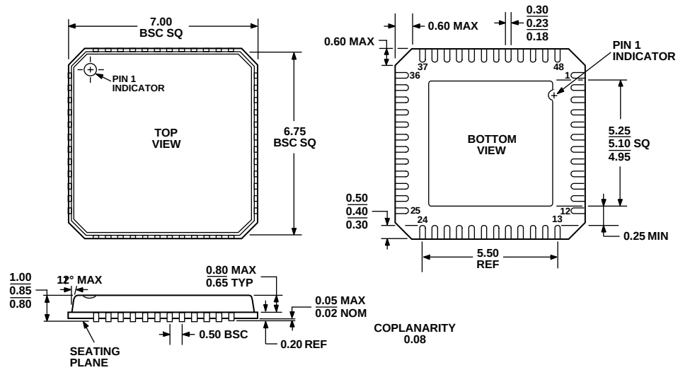
COMPLIANT TO JEDEC STANDARDS MO-220-VKKD-2 Figure 27. 48-Lead Lead Frame Chip Scale Package [LFCSP] 7 mm x 7 mm Body (CP-48) Dimensions shown in millimeters
