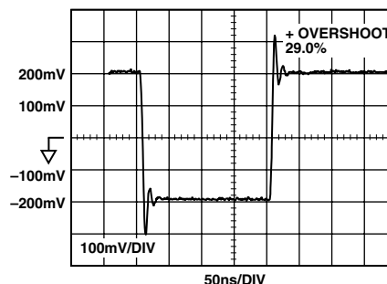
Figure 5. Typical Pulse Response with C_L = 65 \text{ pF} , Gain = +2, and V_S = \pm 2.5 \text{ V}
